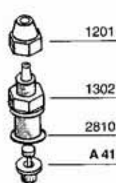
VALVOLA KALREZ KALREZ VALVE
