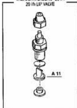
VALVOLA A LABBRIO 20 l/h 20 l/h LIP VALVE
